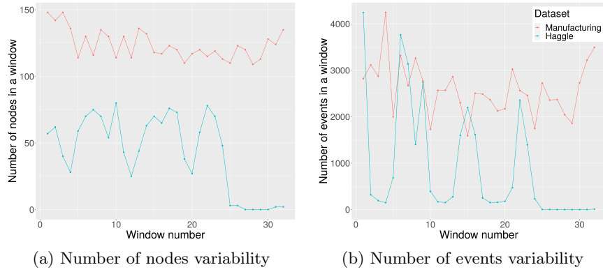
Fig. 2. Number of nodes and number of events for each time window for evaluated datasets: manufacturing company and Haggie for 32 windows.
