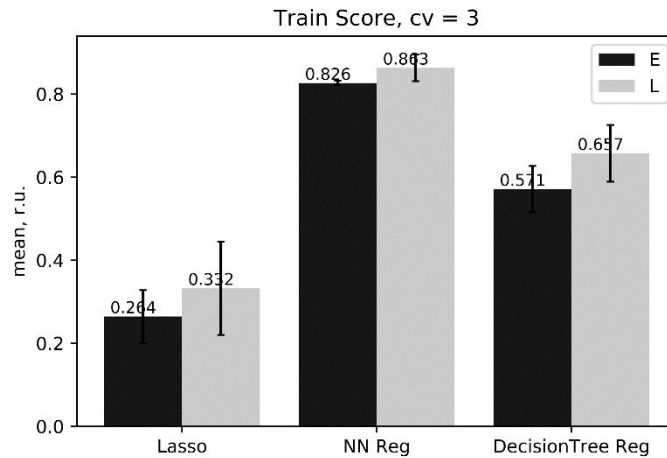
Fig. 4. Mean training scores for the three models with k-fold number cv = 3
