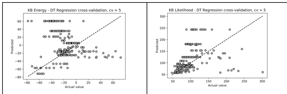
Fig. 3. Decision tree regression cross-validation, k = 5
