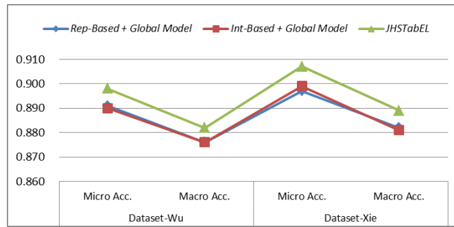
Fig. 5. The performance of different semantic matching models.
