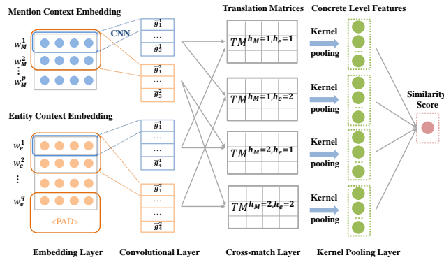
Fig. 4. The Architecture of Interaction-Based Model Using Conv-KNRM.
