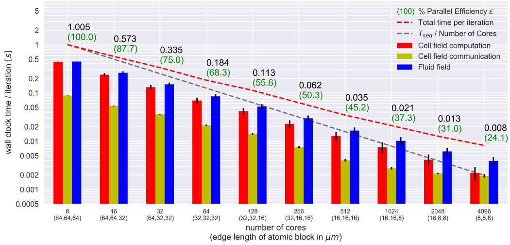
Fig. 7. Statistics for each of the simulations. The fluid part is handled by Palabos. The dotted line shows perfect linear scaling. a) shows the statistics for the naïve implementation of the communication. b) shows the statistics for our improved implementation.
