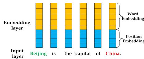
Fig. 2. A Example of word representations with word and position embedding.
