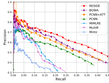
Fig. 4. The PR curves of RESIDE(source from [17])
