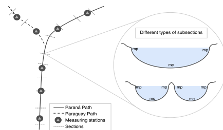
Fig. 1. Discretization of the river domain. Some types of Su in the cross Sc of the domain.
